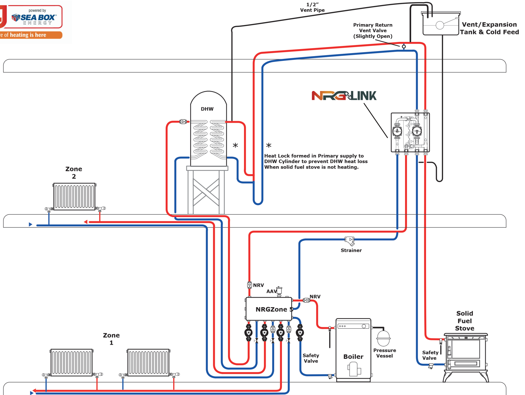
NRG Zone - System Schematic - 67
