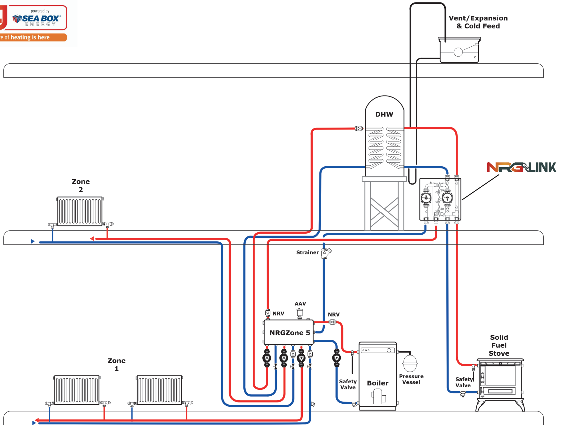
NRG Zone - System Schematic - 65
